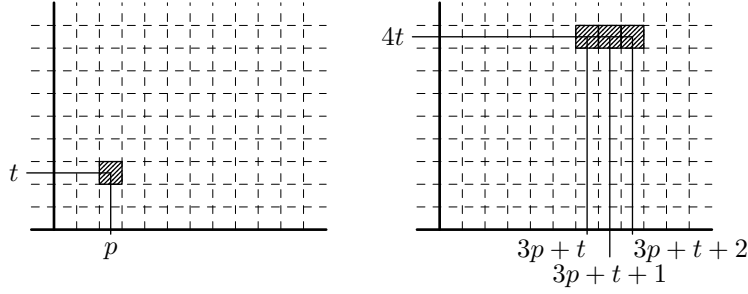
Fig. 10. Sample geometrical transform: (3, \mathbf{\Lambda}^{(3,4,1)})
