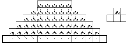
Fig. 9. dependencies in space-time diagrams for grouping
