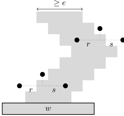
Figure 3: Blocking word w of width e for a CA of neighborhood [r, s] . The gray region represents the consequences of w .
