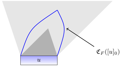
Figure 1: Consequences of a word u .
