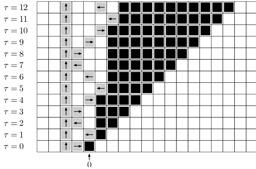
Figure 7: The set \mathcal{P}_0 is exactly the set of sites in state \blacksquare .
