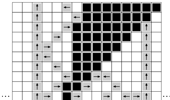
Figure 6: A space-time diagram of the described automaton on an example starting configuration.
