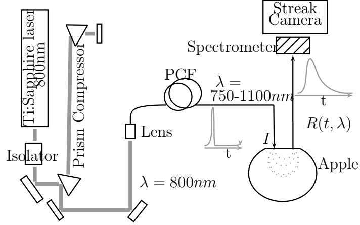
Figure 1: Setup for TRS spectrum acquisition
