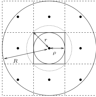
Figure 1: Truncated Z^2 lattice ( k = 1 ). The squares symbolise the Voronoi cells and the dots symbolize the employing high dimension lattices.
