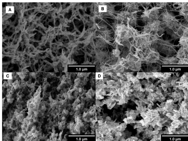
Figure 1. SEM pictures of the cross section of aerogels prepared using the procedure of \text{Eu}^{3+} incorporation: (A) chitosan; (B) Eu–Ch; (C) Eu–ChS–b–H; (D) Eu–ChS–“ in-situ ”–H.
