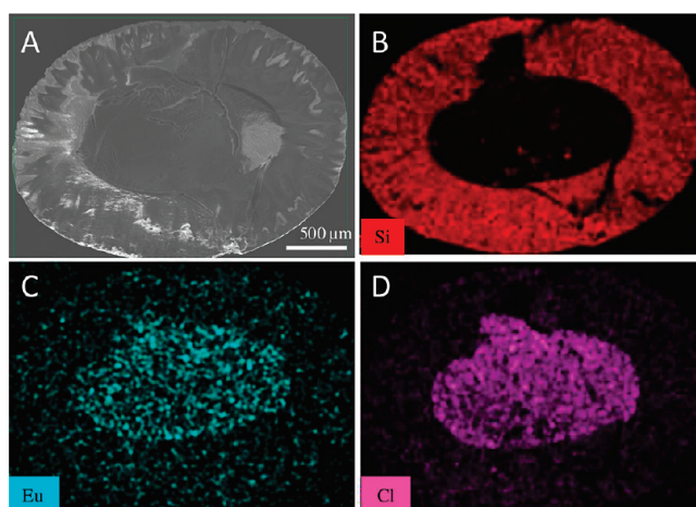
Figure 3. SEM of cross section micrographs of EuChS–CS2 (A). X-ray mapping of the relative Si, Eu, and Cl content in the shell and in the core (B, C, and D, respectively).
