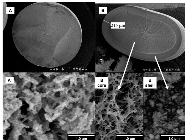
Figure 2. SEM of cross sections of EuChS–H (A, A') and EuChS–CS (B, Bcore, Bshell).
