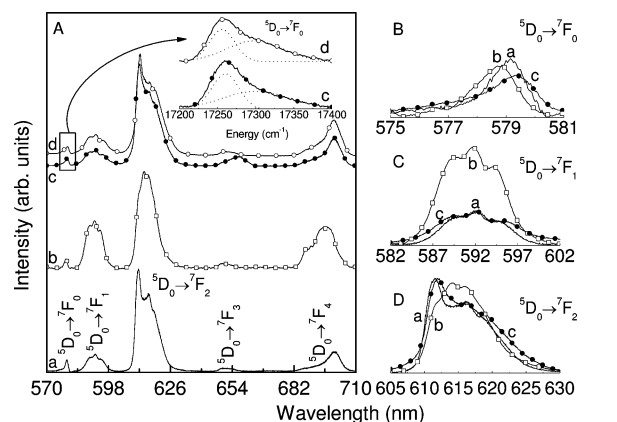
Figure 8. (A) Low-temperature (12 K) intra- 4f^6 emission of the (a) EuCh, (b) EuChS–H, (c) EuChS–CS1, and (d) EuChS–CS2 materials excited at 280 nm. The inset shows in detail the ^5\text{D}_0 \rightarrow ^7\text{F}_0 line for the core–shell hybrids with the respective best fit using a sum of two Gaussian functions. (B, C, D) Detailed view of the ^5\text{D}_0 \rightarrow ^7\text{F}_{0-2} transitions, respectively.
