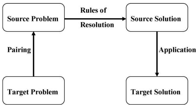
Fig. 5. CBR reasoning [27].
