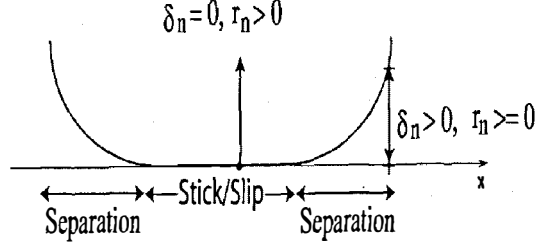
FIGURE 1. Potential contact zone.
