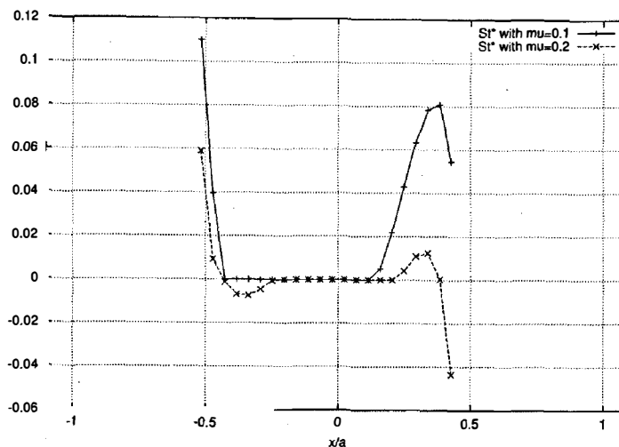
FIGURE 6. Tangential velocity in the effective contact zone: Dependence on the friction coefficient
