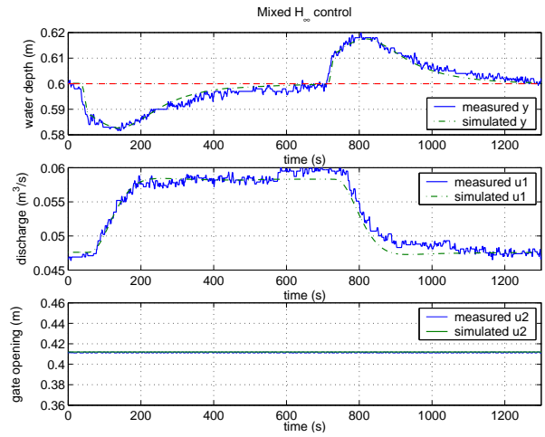
Fig. 9. Experimental response of the distant downstream H_\infty controller 1 to a downstream withdrawal, comparison with a linear simulation
