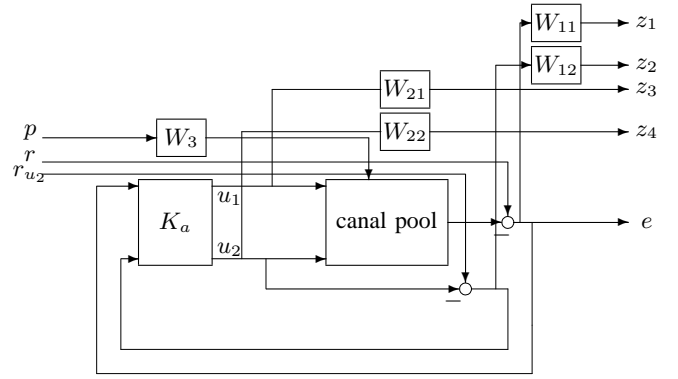
Fig. 6. Augmented system for H_\infty optimization
