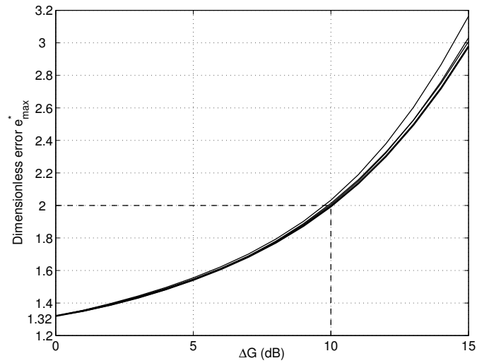
Figure 8: Dimensionless maximum error as a function of \Delta G and different values of the phase margin ratio \Delta\Phi/\Delta\Phi_{\max} \in [0.5, 0.9] .
