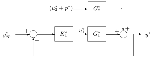
Figure 3: Schematic representation of distant downstream control of a dimensionless canal pool
