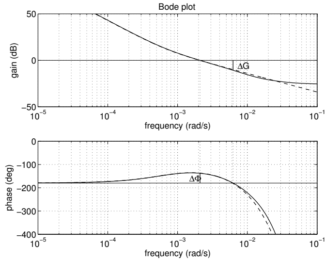
Figure 6: Bode plot of K_1G_1 with the linearized Saint-Venant model (—) and ID model (– –) for pool 4 of ASCE Test Canal 1, high flow conditions.
