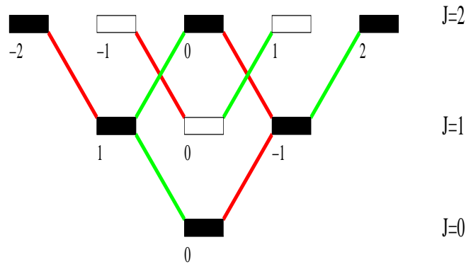
Figure 3. The same conventions as in Fig. 1 are used except that we do not draw on the coupling by D_0 . We note that two connectivity sets appear: those connected with |Y_0^0\rangle (filled black rectangles) and those connected with |Y_1^0\rangle (empty rectangles).
