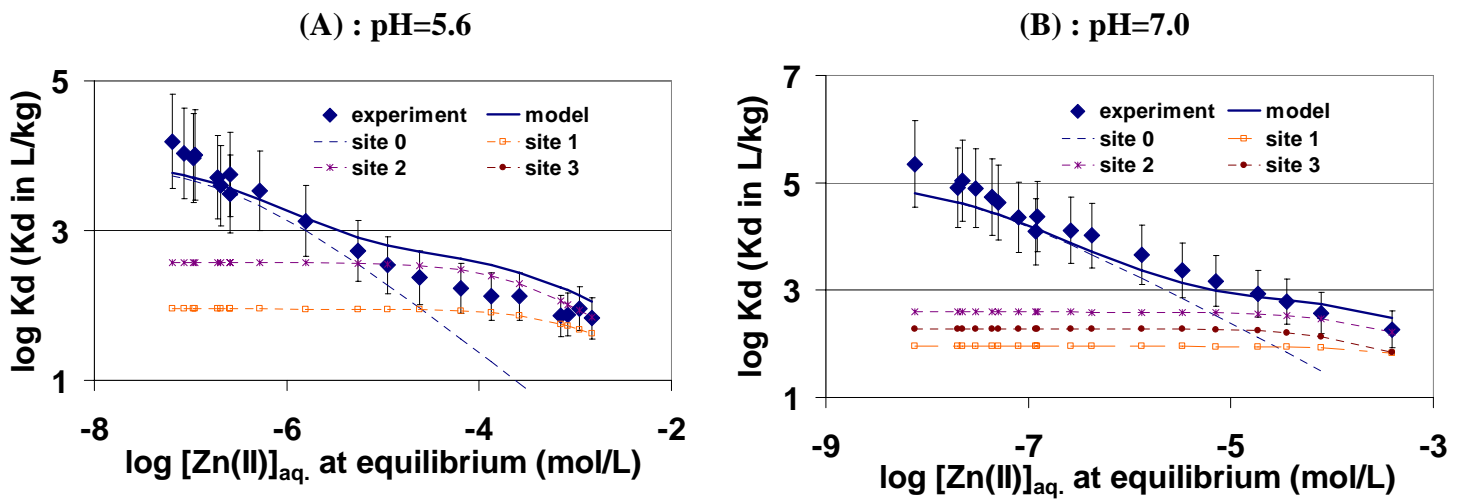
Figure 3: Logarithm of the distribution coefficients of Zn(II) between Wyoming montmorillonite and 0.1 M NaClO 4 solutions as a function of the aqueous zinc concentration at equilibrium and for different pH (A: pH=5.6; B: pH=7.0). Symbols refer to experimental measurements of Baeyens and Bradbury (1997), whereas curves indicate ion-exchange modelling which includes site “0”, the site having low density and strong affinity.
