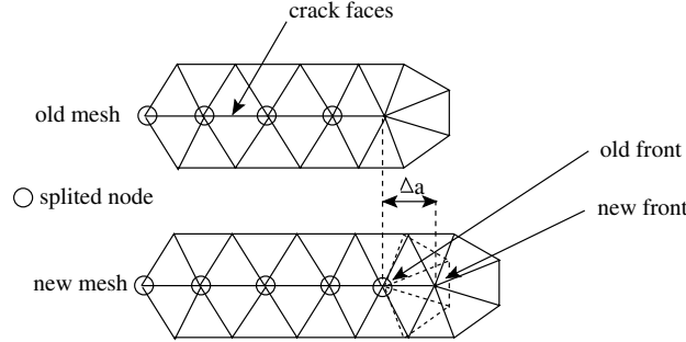
Fig. 5. Remeshing procedure.
