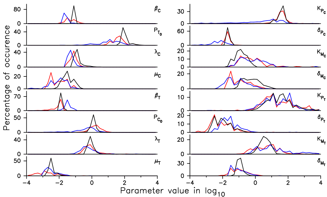
Figure S1: Probability distribution for parameter values in parameter sets with adjustment RMS error below 10%. Parameters are determined as explained in Methods. The percentage of occurrence is evaluated for bins of width 0.2 in \log_{10} . The probability distributions of parameter values for the model with all parameters modulated are shown in red and blue for the day and night values, respectively. The probability distribution of parameter values for the model with all parameters constant is shown in black.
