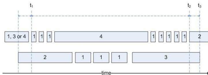
Fig. 5-1. Type i(1) Packets (First Row) and Type i(2) Packets (Second Row). The Left and Right Sides of the Packets are Aligned with Their Starting and Finish Time. The Numbers inside the Packets are the Positions of the Assigned Paths in the Corresponding Path Ordering.
