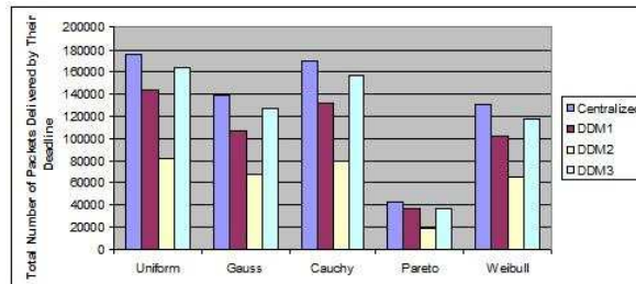
Fig. 4-4. Test Results – Unreliable Data Transfers.
