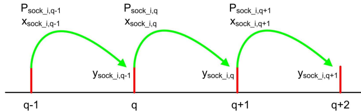
Fig. 3-10. Computation Steps of the Fairness Decisions Module (for Each Socket sock\_i ).
