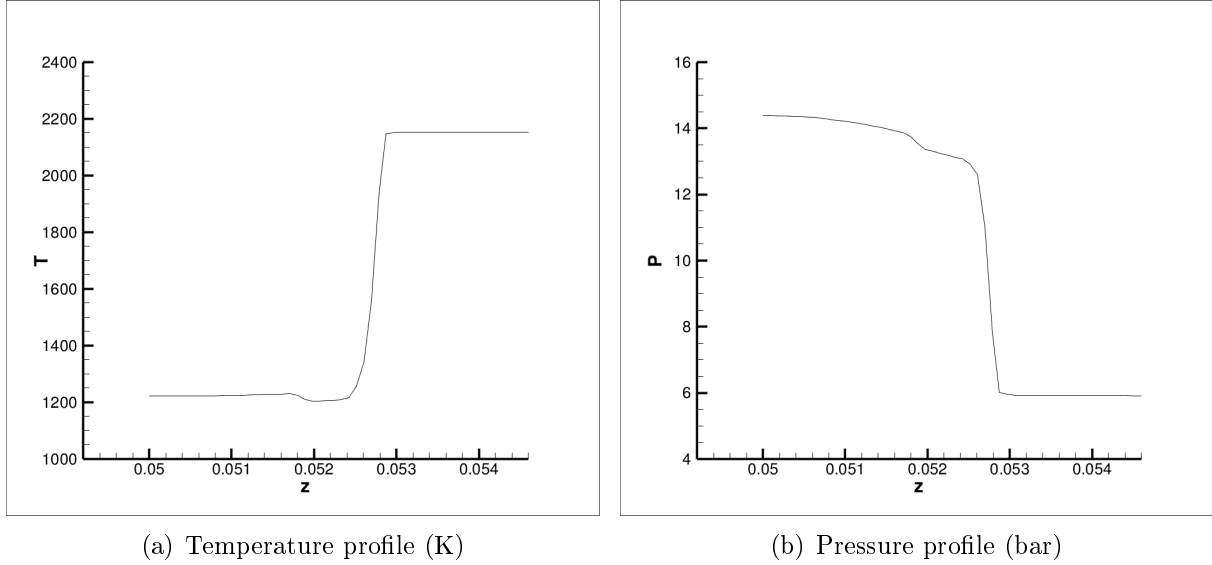
Figure 2. Profile of the shock after plasma heating at time 3\mu s . We see that the flow conditions inside the bow shock impedes the fluid heating in this area.
