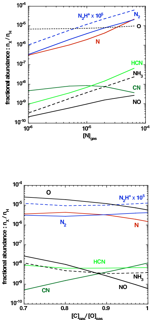
Fig. 7. Steady-state fractional abundances of nitrogen-containing species for a density n_{\text{H}} = 10^4 \text{ cm}^{-3} , a kinetic temperature T = 10 \text{ K} , and a cosmic ray ionization rate of \zeta = 10^{-17} \text{ s}^{-1} . Upper panel: C:O=0.97 is held constant and the gas-phase nitrogen fractional abundance [\text{N}]_{\text{gas}} = n(\text{N})/n_{\text{H}} is varied from 10^{-6} to 6.4 \times 10^{-5} . Lower panel: [\text{N}]_{\text{gas}} = 10^{-5} is held constant and the gas-phase C:O ratio is varied by changing [\text{O}]_{\text{gas}} .
