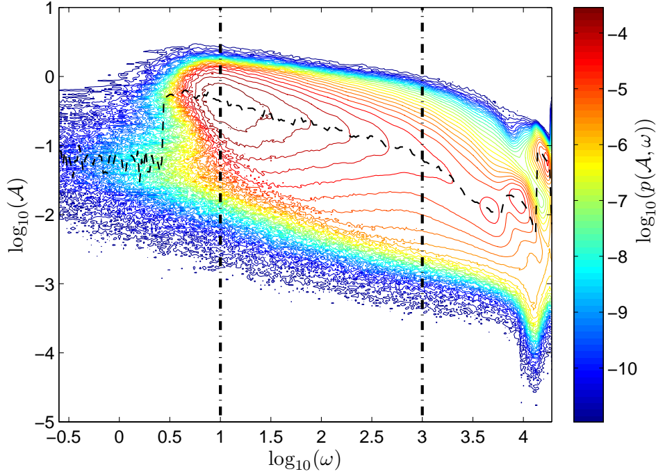
Fig. 4: Representation of the joint pdf p(\omega, \mathcal{A}) (in log scale) of turbulent fluctuations in an amplitude-frequency space. The scaling range 10 < \omega < 1000 Hz for frequencies is shown as vertical dotted lines. The dashed line shows the skeleton \mathcal{A}_s(\omega) of the joint pdf, which is the amplitude for which the conditional pdf p(\mathcal{A}|\omega) is maximum.
