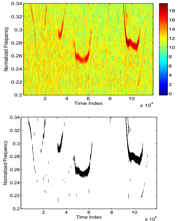
Fig. 4. Whistle of a dolphin. The spectrogram (top) is limited to the normalized frequency [0.2, 0.34] to have a white Gaussian noise on the coefficients. Bottom, detection of signal with a probability of false alarm of 10^{-3} .
