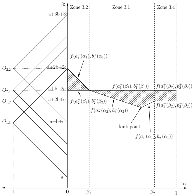
Fig. 12. Output evolution according to \alpha_1
