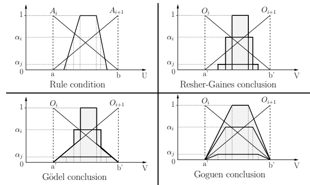
Fig. 6. Inference with two gradual implicitive rules and a fuzzy input decomposed on three levels \alpha_j < \alpha_i < 1
