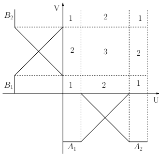
Fig. 9. Areas defined by input partitions
