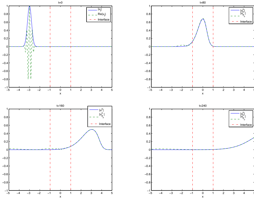
Figure 1: Case V = 0 : modulus of the functions u_{\theta_0}^n and u^n at different time t with x_0 = -3 and \theta_0 = 0.09i
