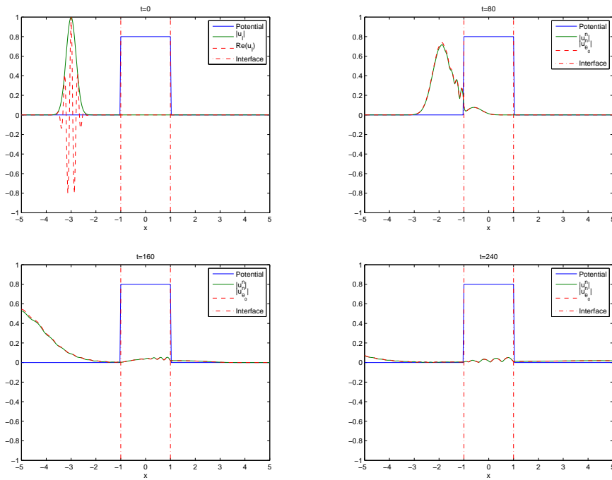
Figure 2: Case of a barrier potential: modulus of the functions u_{\theta_0}^n and u^n at different time t with x_0 = -3 and \theta_0 = 0.09i
