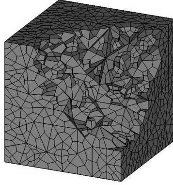
(b) Polyhedral set \mathcal{P}_2
