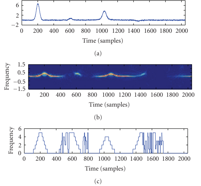
FIGURE 17: (a) Signal s noised at SNR = 20 db; (b) IFL obtained by GCD; (c) associated detection curve.
