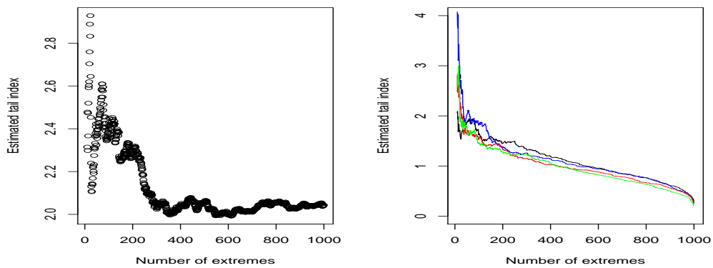
Figure 3: Hill estimator: \alpha = 2 and Pareto iid (left panel), \tau = 1 (right panel); color codes: black - d = 0 , blue - d = 0.2 , red - d = 0.4 , green - 0.45
