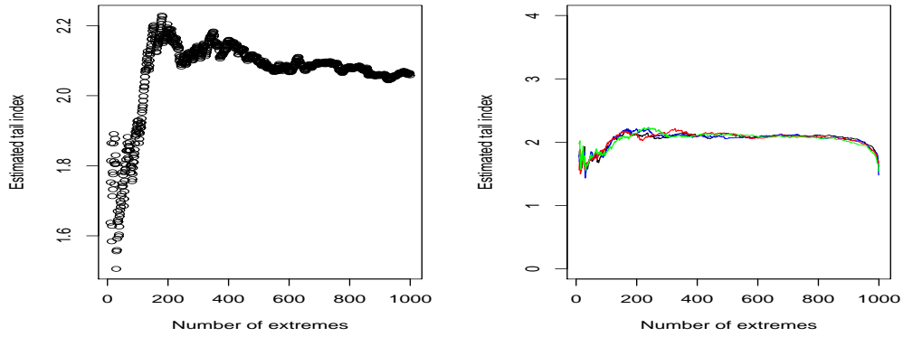
Figure 2: Hill estimator: \alpha = 2 and Pareto iid (left panel), \tau = 0.05 (right panel); color codes: black - d = 0 , blue - d = 0.2 , red - d = 0.4 , green - 0.45
