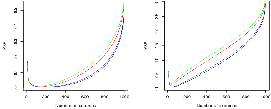
Figure 1: MSE: \alpha = 1 (left panel), \alpha = 2 (right panel); color codes: black - d = 0 , blue - d = 0.2 , red - d = 0.4 , green - 0.45
