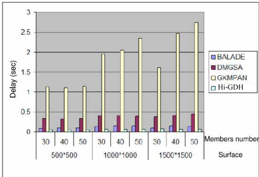
Fig. 3: Average delay of key transmission (seconds)
