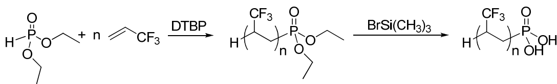
Scheme 6. Radical telomerization of 3,3,3-trifluoropropene (TFP) with diethyl hydrogenophosphonate followed by hydrolysis.
