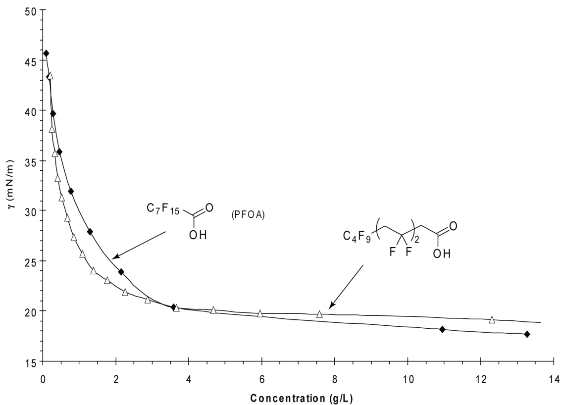
Figure 4: Surface tension measurement of C_4F_9-(VDF)_2-CH_2-COOH (white triangles) compared to PFOA (black diamonds).
