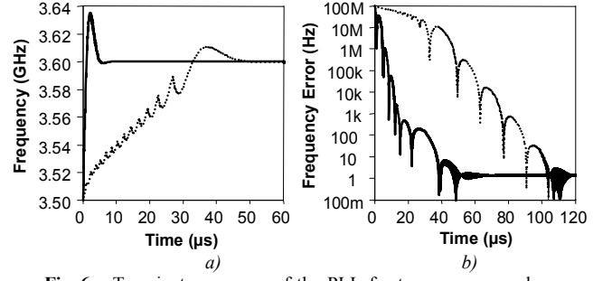
Fig. 6. Transient responses of the PLL for two cases: speed-up mode enabled/disabled (solid/dotted line respectively). Plot b) displays the absolute frequency error in reference to the settling frequency of 3.6 GHz.
