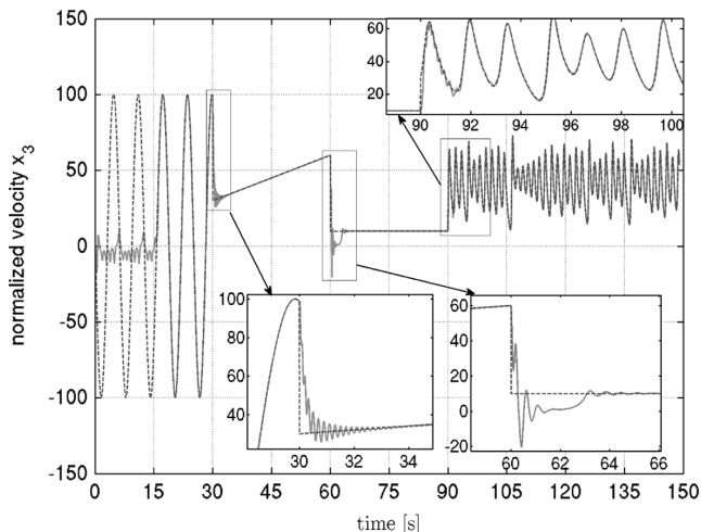
Fig. 4. Simulation under uncertainty and noise. Graph of the normalized angular velocity, i.e., x_3 and its reference trajectory. Zooms on reference changes are also shown. Actual response shown in solid line, reference in dashed line.
