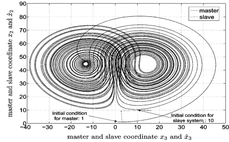
Fig. 4. Lorenz slave and master systems: phase portrait of x_2 versus x_3 (master, continuous line) and \hat{x}_2 versus \hat{x}_3 (slave -dotted line).
