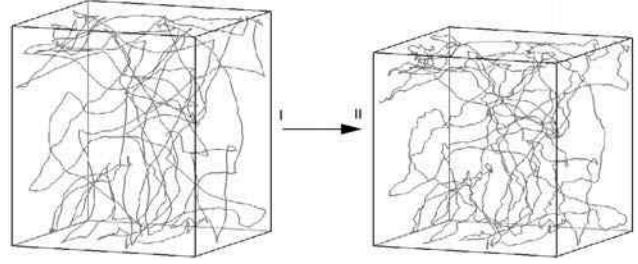
Fig. 7 Tortuosity evolution of a wire network before (I) and after (II) a deposit under gravity from \xi_I = 839 \text{ m}^{-1} to \xi_{II} = 1464 \text{ m}^{-1} .
