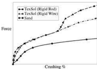
Fig. 4 Biaxial test of sand and TexSol TM 2D samples using unilateral and bilateral laws [16].
