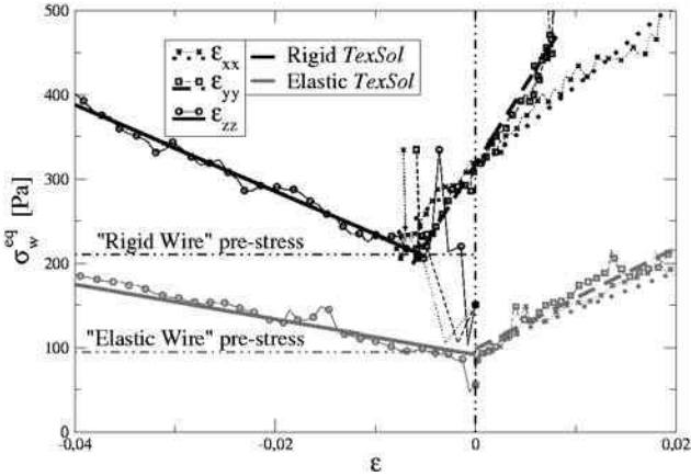
Fig. 15 Wire equivalent stress vs. strains plots for TexSol TM samples.
