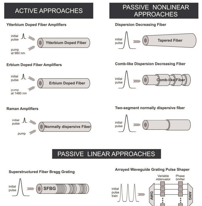
Fig. 6. Various active and passive approaches for parabolic pulse generation
