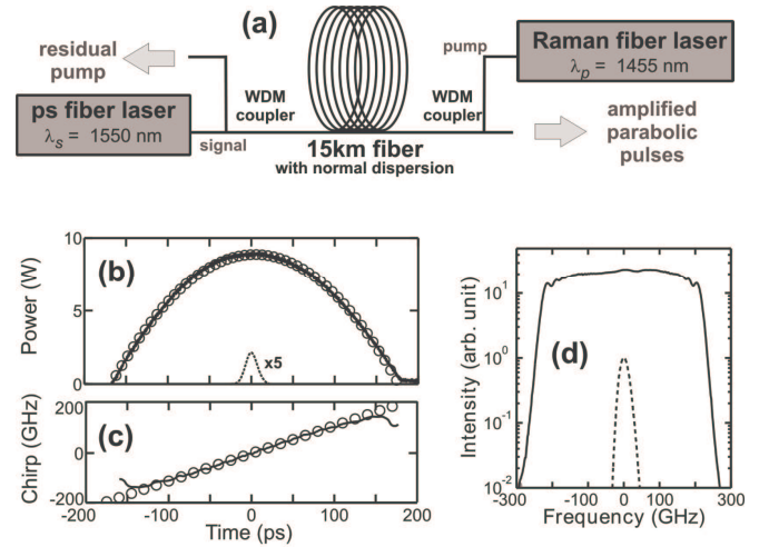
Fig. 4. Generation of parabolic pulses through Raman amplification at telecommunication wavelength (a) Experimental set-up (b) Intensity profiles of the initial pulse (dotted line) and output pulse (solid black line) compared with a parabolic fit (circles) (c) Chirp of the output pulse compared with a linear fit (circles) (d) Spectrum of the initial and output pulses (dashed and solid lines respectively). Results adapted from [53].
