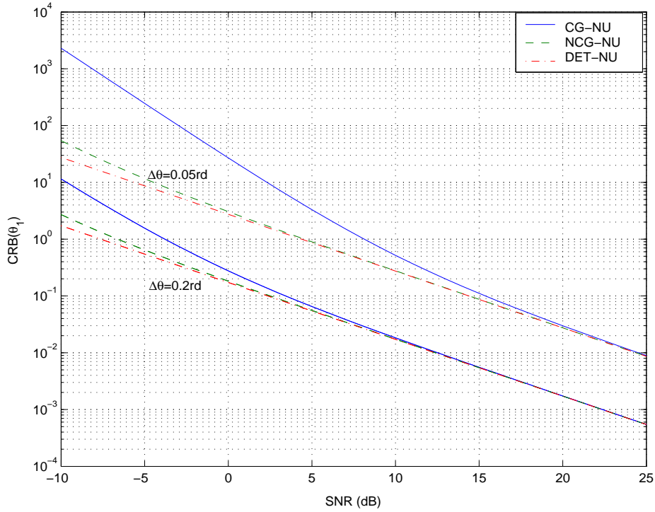
Fig.2 \text{CRB}_{\text{NU}}^{\text{NCG}}(\theta_1) , \text{CRB}_{\text{NU}}^{\text{CG}}(\theta_1) and \text{CRB}_{\text{NU}}^{\text{DET}}(\theta_1) as a function of the SNR for two values of the DOA separation with \Delta\phi = 0.52rd .
