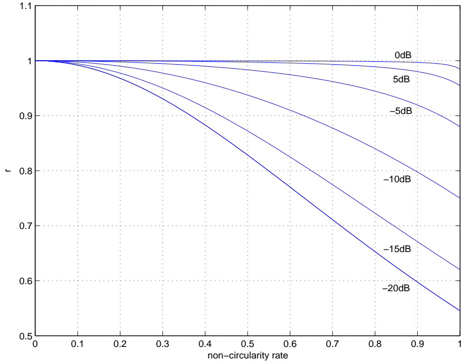
Fig.3 Ratio r \stackrel{\text{def}}{=} \frac{\text{CRB}_{\text{NU}}^{\text{NCG}}(\theta_1)}{\text{CRB}_{\text{NU}}^{\text{CG}}(\theta_1)} as a function of the non-circularity rate \rho_1 for different values of the SNR.
