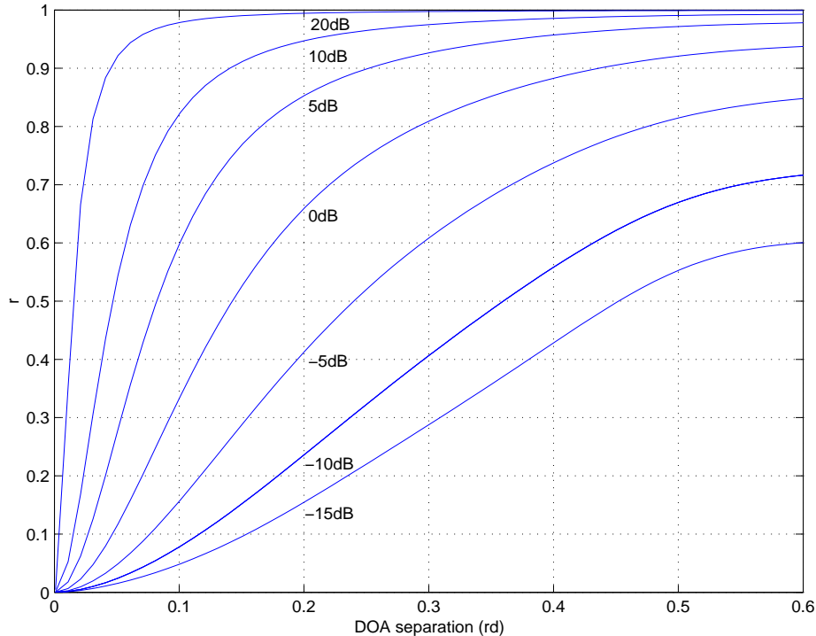
Fig.5 Ratio r \stackrel{\text{def}}{=} \frac{\text{CRB}_{\text{NU}}^{\text{NCG}}(\theta_1)}{\text{CRB}_{\text{NU}}^{\text{CG}}(\theta_1)} as a function of the DOA separation for different values of SNR with \rho_2 = \rho_1 = 1 and \Delta\phi = 0.52rd .
