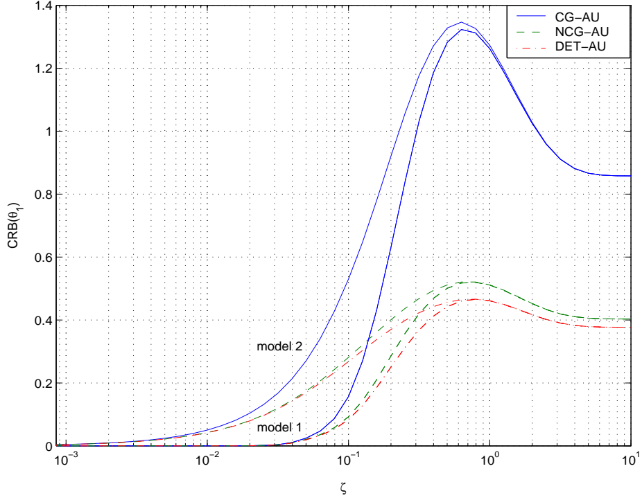
Fig.1 \text{CRB}_{\text{AU}}^{\text{NCG}}(\theta_1) , \text{CRB}_{\text{AU}}^{\text{CG}}(\theta_1) and \text{CRB}_{\text{AU}}^{\text{DET}}(\theta_1) as a function of \zeta for the first and second models with \Delta\theta = 0.1rd , \text{SNR} = 0dB and \Delta\phi = 0.52rd .
