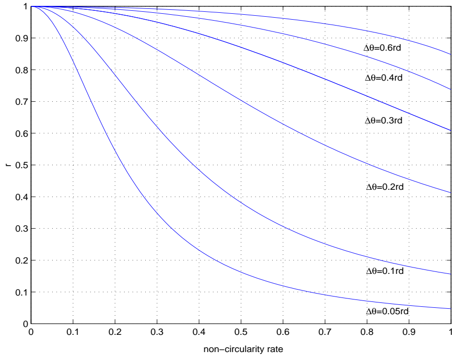
Fig.4 Ratio r \stackrel{\text{def}}{=} \frac{\text{CRB}_{\text{NU}}^{\text{NCG}}(\theta_1)}{\text{CRB}_{\text{NU}}^{\text{CG}}(\theta_1)} as a function of the non-circularity rate for different values of DOA separation with SNR= -5dB and \Delta\phi = 0.52rd .
