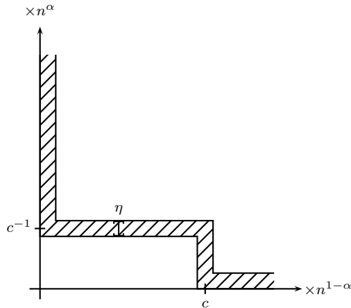
FIGURE 2. Limit shape of a rescaled random diagram under the Schur-Weyl measure of parameters c > 0 and \alpha < 1/2 .
