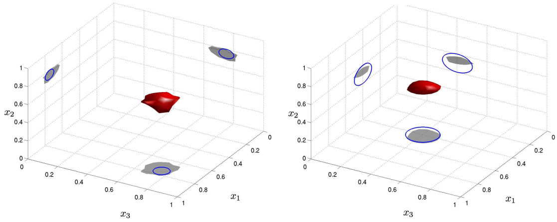
(a) R = 0.05 , \epsilon = 0.6 (b) R = 0.1 , \epsilon = 0.6
