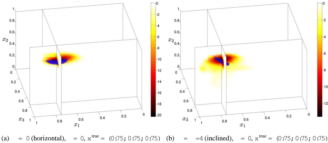
Figure 21: Penny-shaped crack identification: thresholded TS field T .
