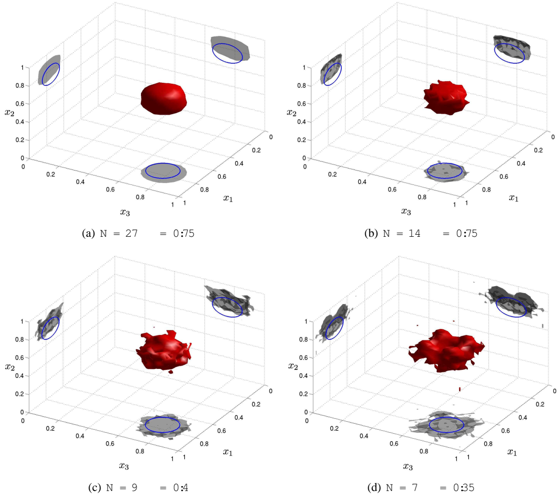
Figure 17: Influence of measurement grid density: blurring effect on B_{eq}(\cdot) .
