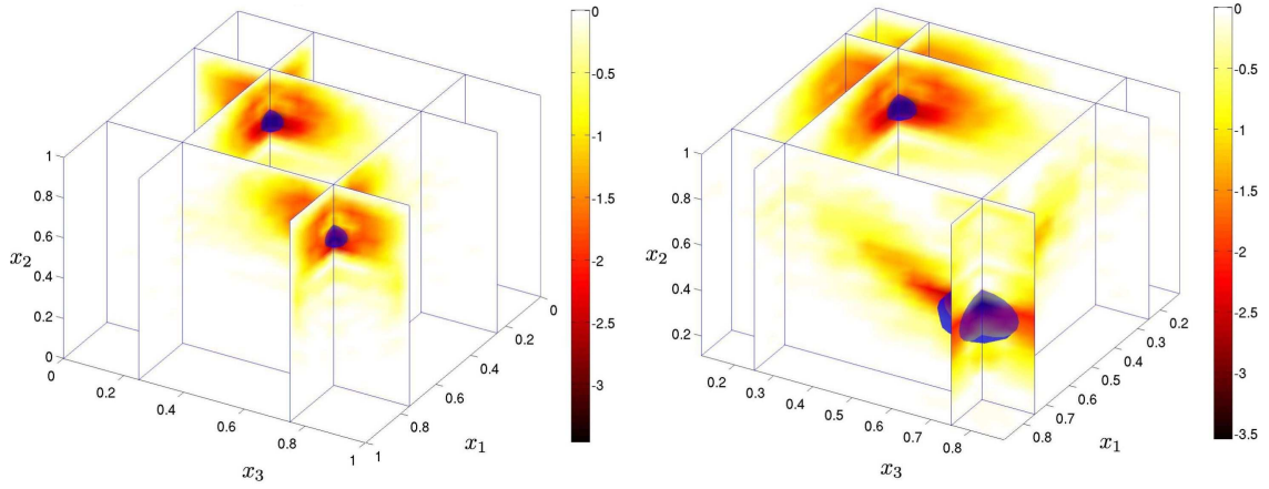
(a) R_1 = R_2 = 0.05 , x_1^{\text{true}} = (0.25; 0.25; 0.75) , x_2^{\text{true}} = (0.75; 0.75; 0.75) (b) R_1 = 0.05 , R_2 = 0.1 , x_1^{\text{true}} = (0.25; 0.25; 0.75) , x_2^{\text{true}} = (0.75; 0.75; 0.5)
