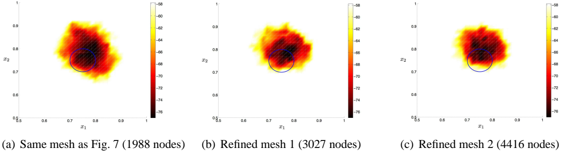
(a) Same mesh as Fig. 7 (1988 nodes) (b) Refined mesh 1 (3027 nodes) (c) Refined mesh 2 (4416 nodes) Figure 8: Single cavity identification, 2D ( R_1 = 0:05 , x^{true} = (0:75; 0:75) ): thresholded TS field T with \tau = 0:75 for three different meshes.
