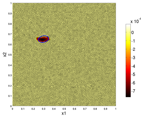
Figure 3: Identification of a single scatterer: distribution of thresholded topological sensitivity \mathbb{T} , with \mathbb{T} = 2 and \epsilon = 1=2 .
