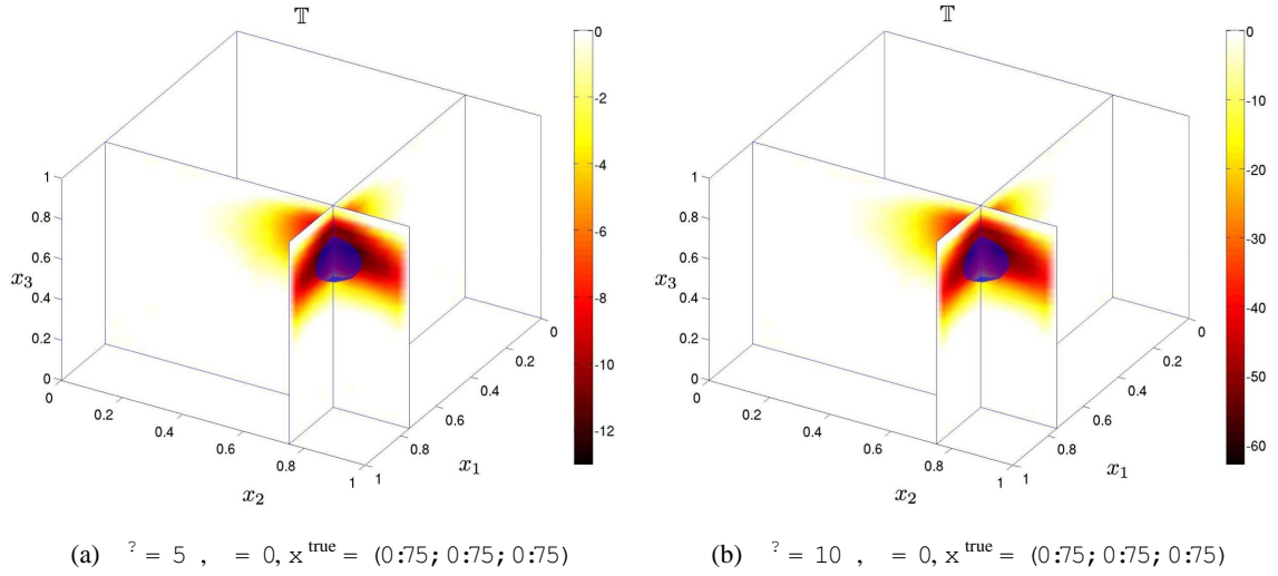
Figure 23: Identification of a stiff spherical inclusion using inclusion-related thresholded TS field \mathbb{T} .
