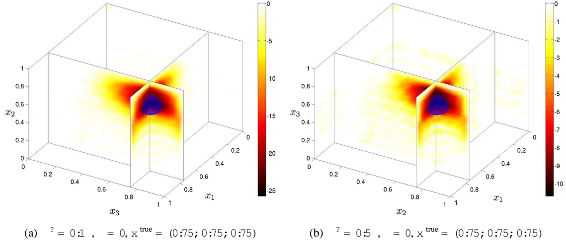
Figure 22: Identification of a soft spherical inclusion using cavity-related thresholded TS field \mathbb{T} .
