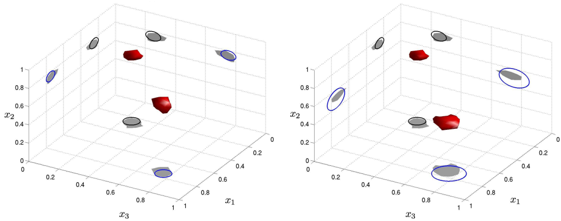
(a) R_1 = R_2 = 0.05 , \epsilon = 0.6 (b) R_1 = 0.05 , R_2 = 0.1 , \epsilon = 0.7
