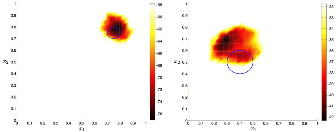
Figure 7: Single cavity identification, 2D: thresholded TS field T with T = 0.75 .
