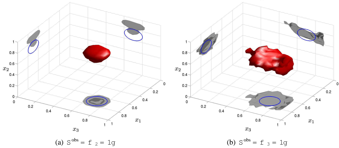
Figure 19: Influence of limited aperture: B_{eq}(\cdot) for two choices of partial observation surface S^{obs} .
