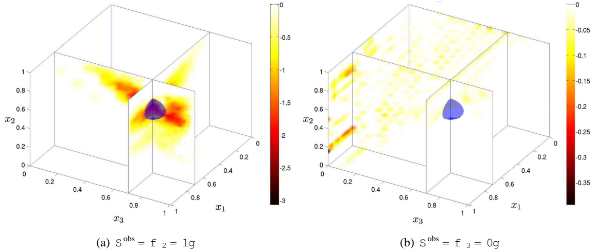
Figure 18: Influence of limited aperture: distribution of T for two choices of S^{obs} .
