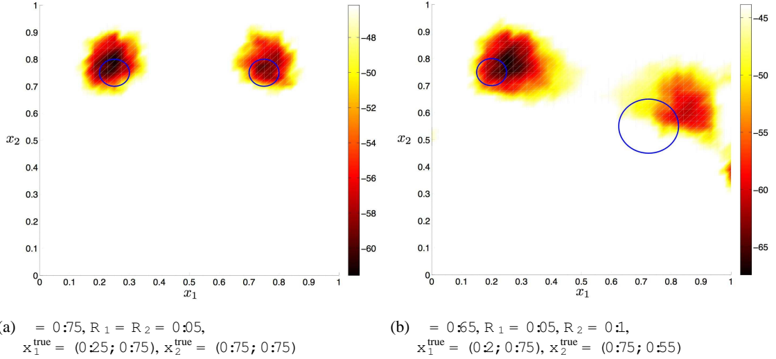
(a) \tau = 0:75 , R_1 = R_2 = 0:05 , x_1^{true} = (0:25; 0:75) , x_2^{true} = (0:75; 0:75) (b) \tau = 0:65 , R_1 = 0:05 , R_2 = 0:1 , x_1^{true} = (0:2; 0:75) , x_2^{true} = (0:75; 0:55) Figure 9: Dual cavity identification, 2D: thresholded TS field T .
