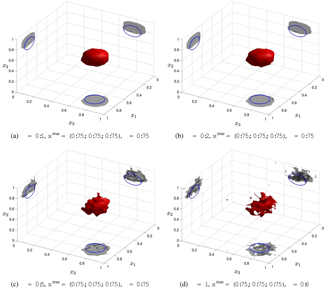
Figure 20: Influence of data noise on T: B_{eq}(\cdot) for various levels of noise.
