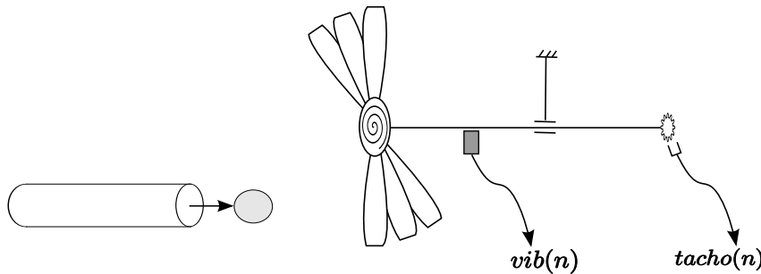
Figure 1: Test rig composed of a single fan with a small number of symmetric blades, and equipped with a tachometer and a vibration sensor.
