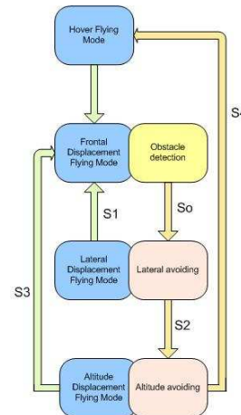
Fig. 3. Overall state machine system
