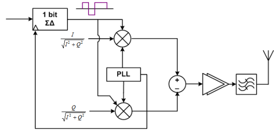
Fig. 7 Polar \Sigma\Delta Architecture
