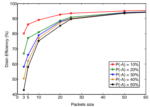
Fig. 4. \eta_D (%) for different packets sizes.
