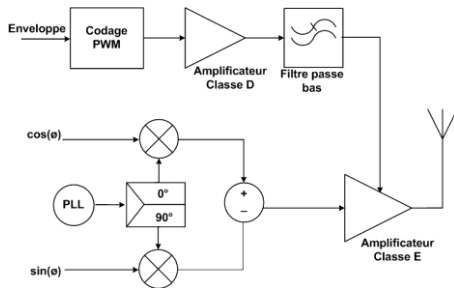
Fig. 6 EER / PWM Transmitter Architecture
