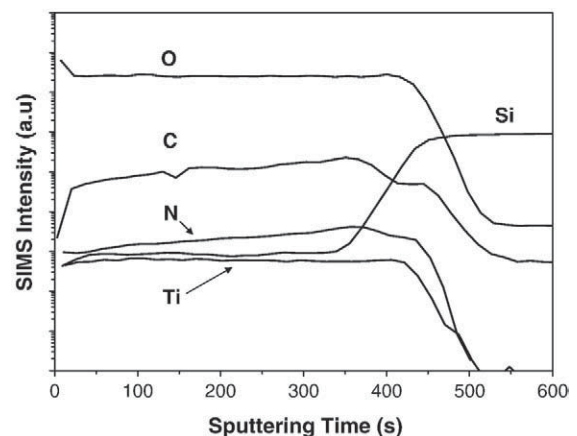
Fig. 5. SIMS profiles of an N-doped TiO 2 film grown on Si(100), at 300 °C, using R=555 (film thickness = 200 nm).
