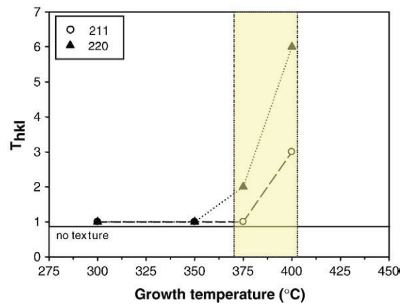
Fig. 4. Variation of texture coefficient in the (211) and (220) direction with the growth temperature for N-doped TiO 2 films grown with R=2200 .
