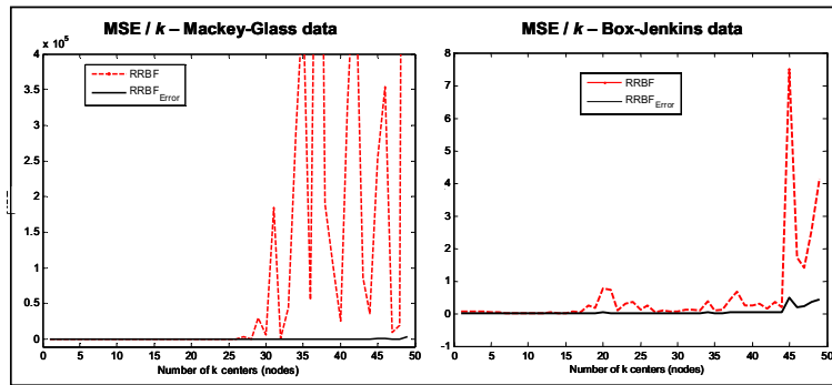
Figure 6. MSE with regards to the number of k centres at " t+1 "
