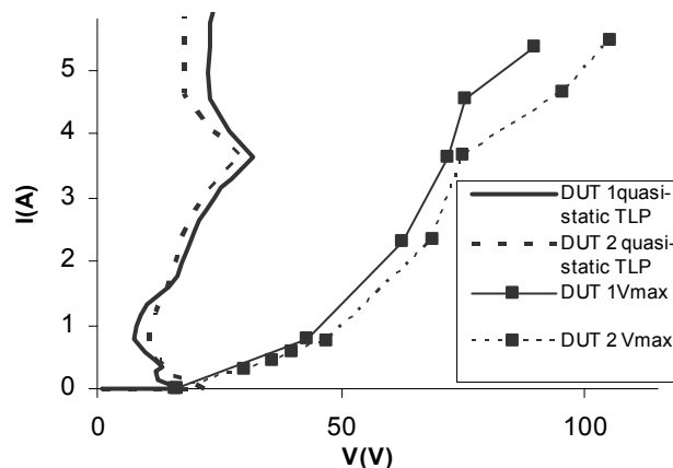
Figure 13: Quasi-static and transient measurements on two NPN devices with different base dopings.
