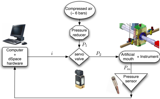
Figure 1. Principle of the pressure controlled artificial mouth. Through a control algorithm implemented on a DSP card, the volume flow through the servo-valve is modified every 40\mu s in order to minimize the difference between the measured and the target mouth pressure.
