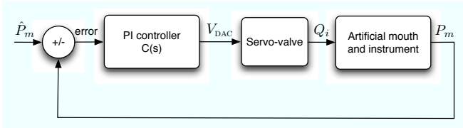
Figure 9. Principle of the pressure controlled artificial mouth. Through a control algorithm implemented on a DSP card, the volume flow through the servo-valve is modified every 40\mu\text{s} in order to minimize the difference between the measured and the target mouth pressure.
