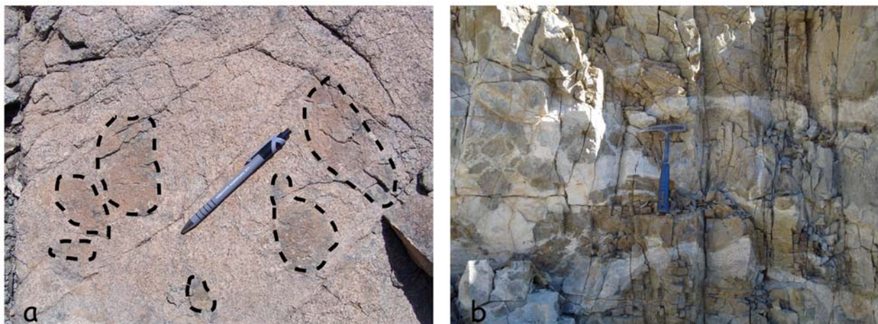
Figure 4. (a) Xenoliths of granoblastic dikes in isotropic ophitic gabbro and (b) magmatic breccia consisting of recrystallized sheeted dike within a silicic (oceanic plagiogranite) matrix. Both outcrops are in the Wadi Gideah area.
