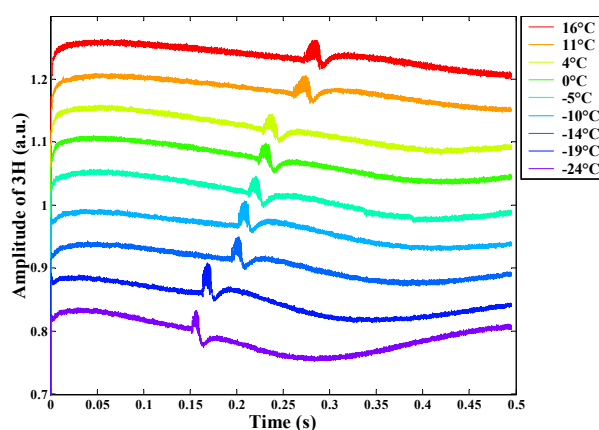
Figure 2: 3H versus low gas temperature
