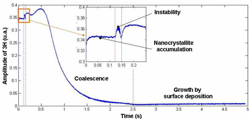
Figure 1: Identification of the different formation steps on the 3H time evolution
