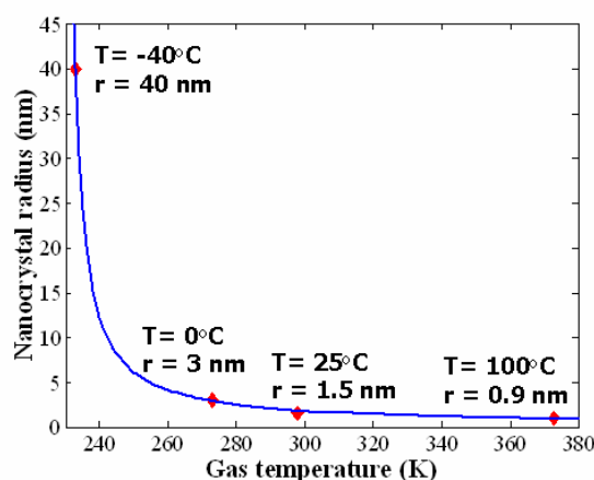
Figure 4: Nanocrystal radius versus gas temperature
