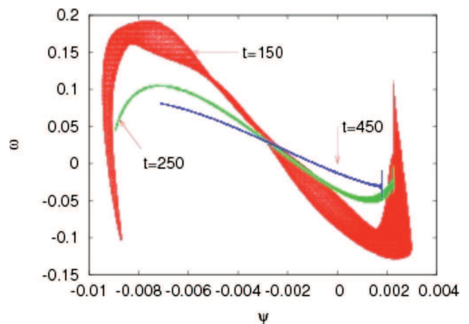
FIG. 10. (Color online) Scatter plot of \omega vs \psi at three different instants in regime I.
