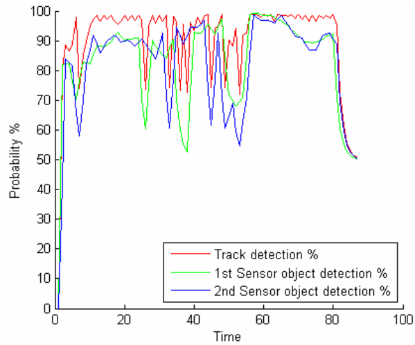
Fig.9. Track detection confidence variation of one pedestrian detected by two sensors having different detection performance.
