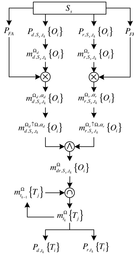
Fig.5. Confidence updating algorithm.
