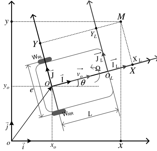
Fig.4. absolute and relative coordinate systems
