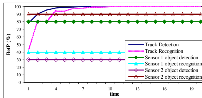
Fig.6. Track detection and recognition with two sensors: confidences follow the powerful sensor up to 100%
