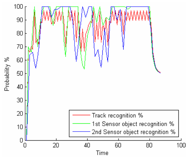
Fig.10. Track recognition confidence variation of one pedestrian recognized by two sensors having different recognition performance.
