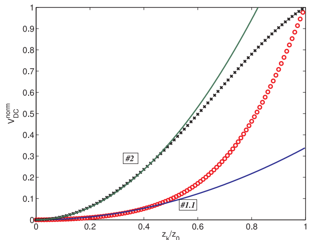
Figure 7: (Color Online) Normalised potentials created by the DC electrodes on axis (0,0,z) for geometries #1 (empty circles) and #2 (crosses) together with their respective fits to f(z) = az^2 (solid lines). Notice that the fit was performed considering only V(z_k \leq 0.5z_0) .
