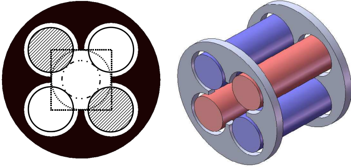
Figure 8: (Color Online) Description of the proposed alternative geometry, #4. The electric connections are the same as for trap #2, see table 1 for details. The DC electrodes geometry has been chosen so that the inner cut corresponds to the circumference inscribed in a square defined by the four rod centres.
