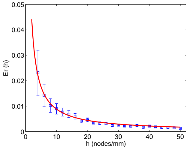
Figure 3: (Color Online) Estimation of the error between the numerical solution given by SIMION8.0 and the known analytical potential in the case of infinite hyperbolic electrodes as a function of the mesh density h . The dots show E_r(h) calculated by equation 4 whereas the curve plots f(h) = a/h , with a = 8.8 \times 10^{-2} . The error bars correspond to 1\sigma .
