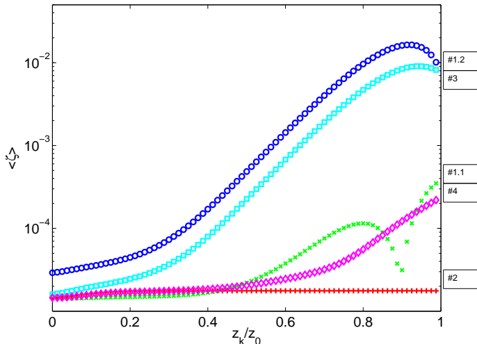
Figure 6: (Color Online) Averaged anharmonic contribution \langle \zeta(z_k) \rangle along the trap axis for the configurations #1.1, #1.2, #2. Configurations #3 and #4 are introduced later in the text. Strong differences between the trap configurations appear from z_k/z_0 > 0.2 . For clarity, only every 4 th node is plotted.
