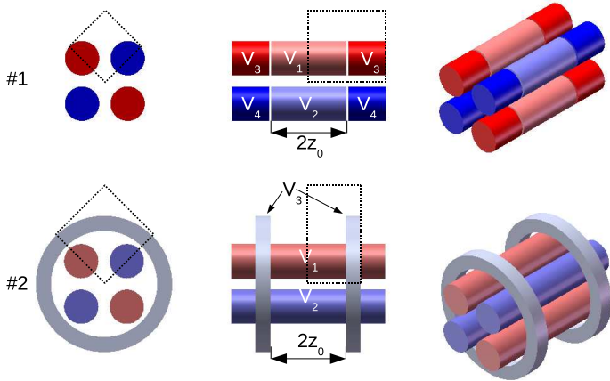
Figure 2: (Color Online) Design of the first two analysed geometries. The dimensions used in both cases are: r_0 = 4 mm and z_0 = 10 mm, with r_e = 1.14511r_0 . Trap #1 is formed by four segmented rods whose electrical connections are detailed in table 1. Trap #2 consists of four continuous rods surrounded by DC electrodes made of two external rings of longitudinal dimension l_{ring} = 4 mm, inner radius r_{int} = (r_0 + 2r_e) + 1 mm and outer radius r_{ext} = r_{int} + 5 mm. The distance between these rings defines 2z_0 . The dotted lines define the volume used for the SIMION8.0 calculations.
