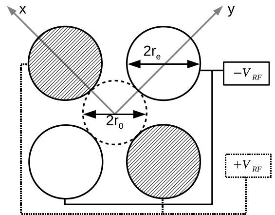
Figure 1: Schematic transverse view of a linear RF trap made of four cylindrical electrodes. The axes convention is shown, as well as the definitions of the applied RF voltages V_{rf} = \frac{U_0 + V_0 \cos \Omega t}{2} , the trap radius r_0 and the electrode radius r_e .
