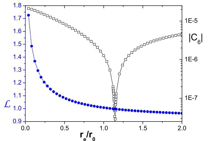
Figure 4: (Color Online) Squares and right axis: absolute value of the first anharmonic coefficient C_6 , versus r_e/r_0 for r_0 = 4 mm. Blue circles and left axis: loss factor, \mathcal{L} versus r_e/r_0 .
