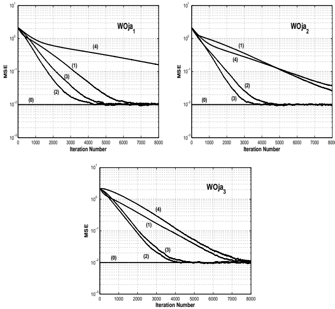
Fig.1 Learning curves of the MSE E\|\mathbf{W}_k - \mathbf{W}\|_{\text{Fro}}^2 averaging 1000 independent runs for the 3 PCA WOja algorithms compared to \mu \text{Tr}(\mathbf{C}_W) (0) for different values 0.9 (1), 0.6 (2), 0.4 (3), 0.1 (4) of \omega_1/\omega_2 for n = 3 , p = 2 and (\lambda_1, \lambda_2, \lambda_3) = (1, 0.6, 0.2) .
