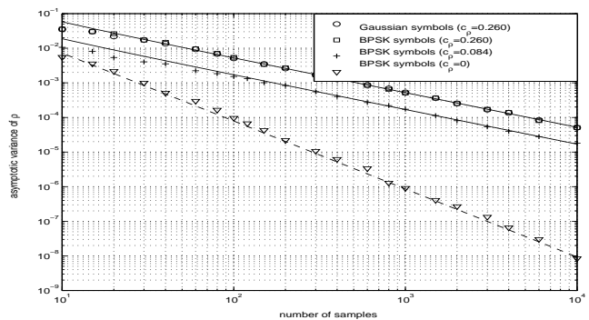
Fig.2 Asymptotic theoretical variance and empirical (averaging 1000 runs) MSE of the estimate \hat{\rho}_T , compared to the asymptotic theoretical variance c_\rho as a function of the number T of observations for Gaussian and BPSK symbols associated with different channels (h_0, h_1) for \rho = 0.7 .
