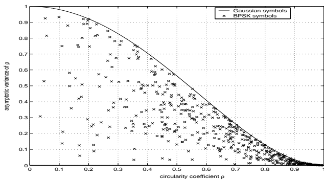
Fig.1 Asymptotic theoretical variance c_\rho given by (3) as a function of the circularity coefficient \rho for BPSK and Gaussian symbols s_t for P = 2 and 500 realizations of a Rayleigh channel whose three coefficients have same variance.
